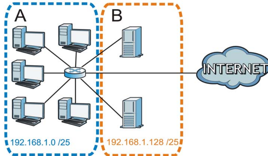
Figure 183 Subnetting Example: After Subnetting
