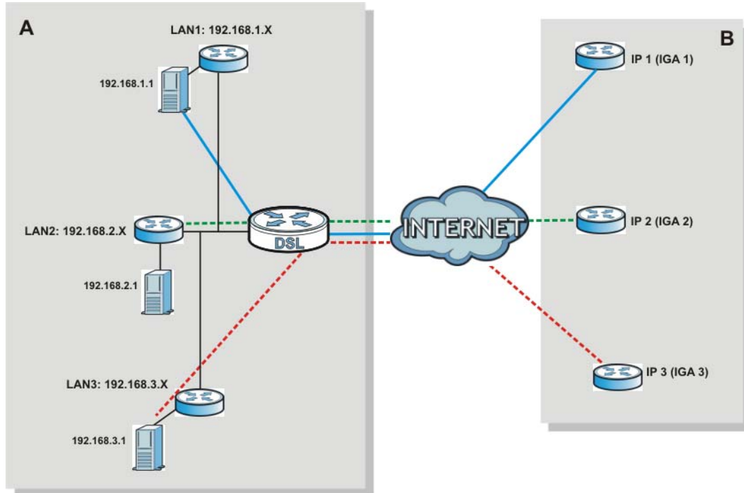
Figure 85 NAT Application With IP Alias
