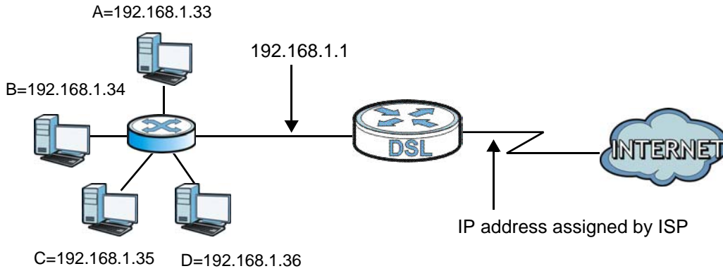
Figure 86 Multiple Servers Behind NAT Example
