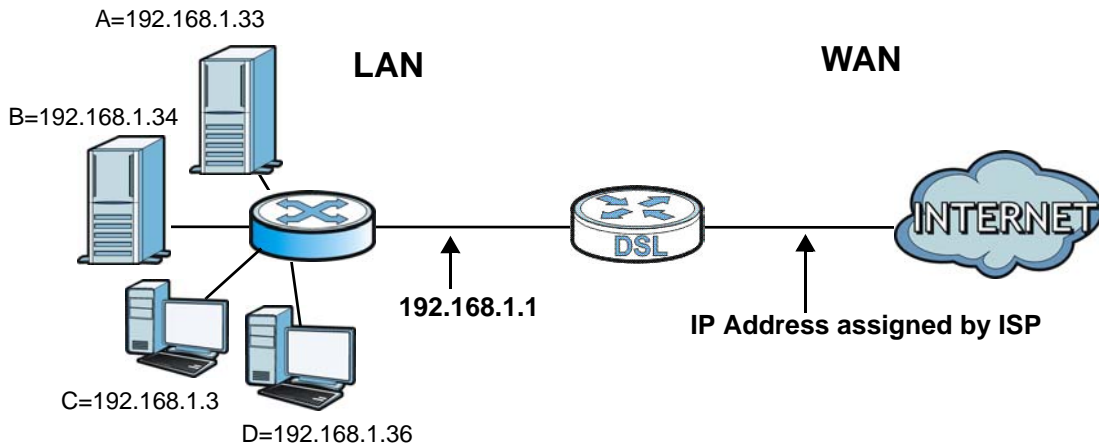
Figure 72 Multiple Servers Behind NAT Example
