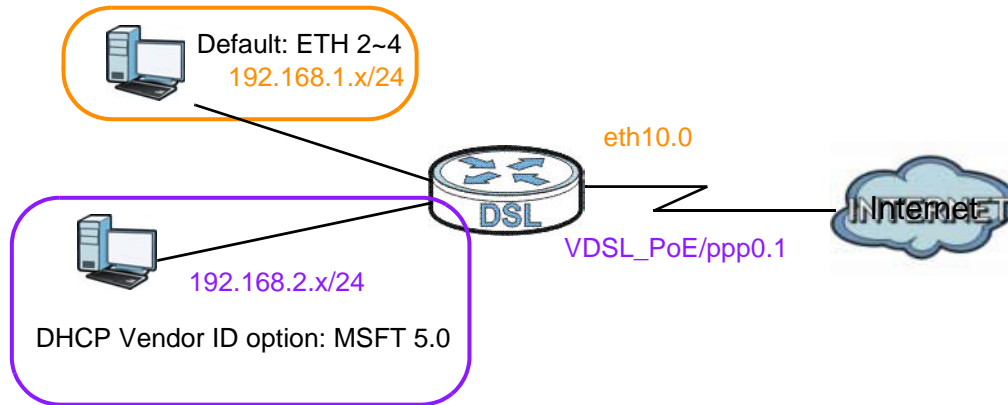
Figure 90 Interface Grouping Application
