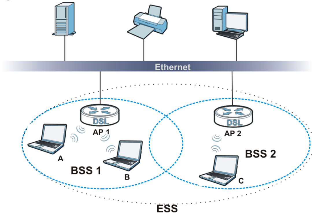
Figure 196 Infrastructure WLAN
