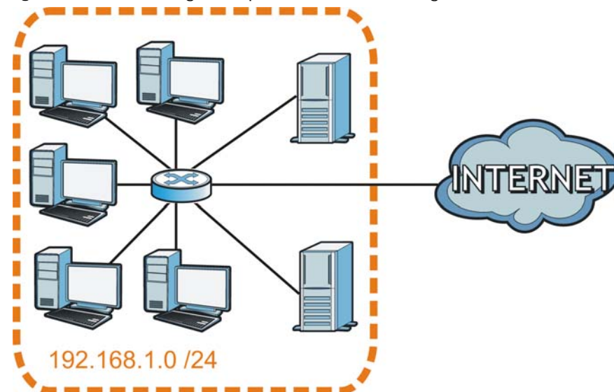
Figure 182 Subnetting Example: Before Subnetting
