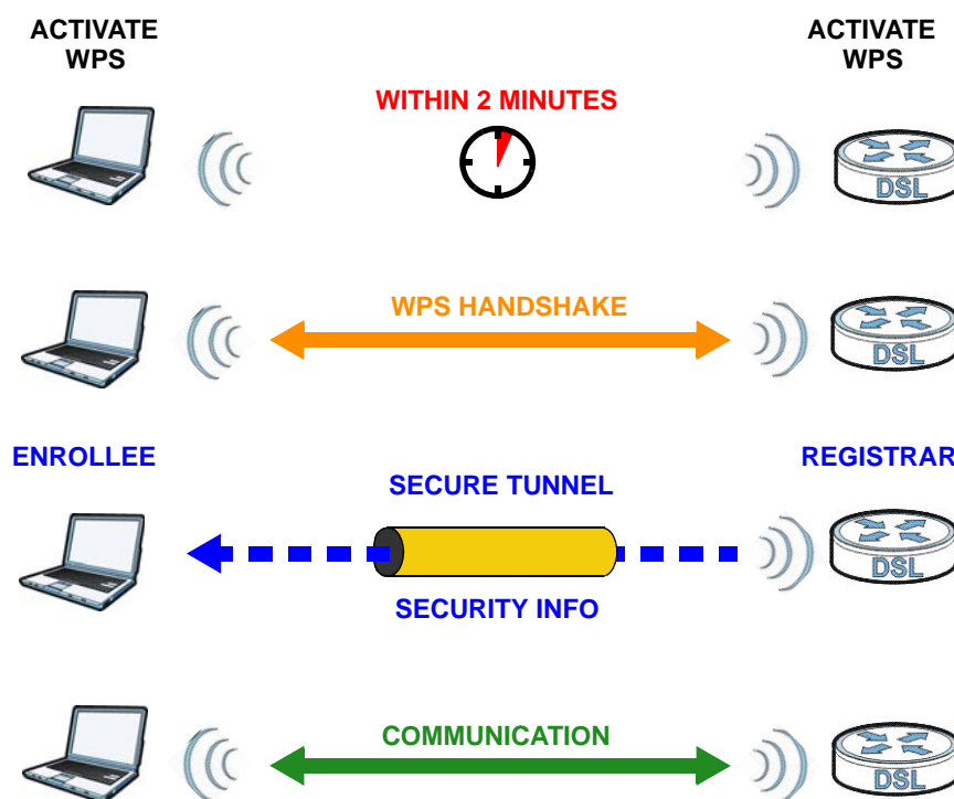
Figure 47 How WPS works
